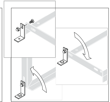
Bodenmontage-Winkel (2er-Set) Floor mounting angle iron (set of 2) Art.-Nr. Item No. 10500002 Preis je Paar € 6.50 Price per pair €
